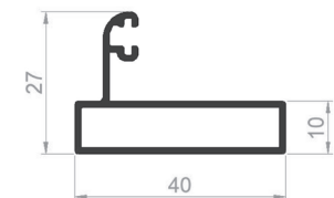
PROFILE CODE: 75400-00 WEIGHT: 0,413 Kg/m
