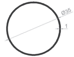
PROFILE CODE: 35041-00 WEIGHT: 0,289 Kg/m
