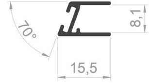
PROFILE CODE: 75460-00 WEIGHT: 0,117 Kg/m
