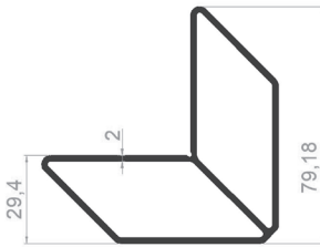
PROFILE CODE: 06954-00 WEIGHT: 1,673 kg/m
