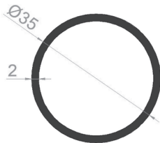
PROFILE CODE: 35098-00 WEIGHT: 0,561 Kg/m
