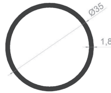
PROFILE CODE: 50296-00 WEIGHT: 0,509 Kg/m
