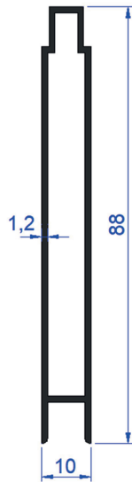
PROFILE CODE: 80001-12 WEIGHT: 0,621 Kg/m
