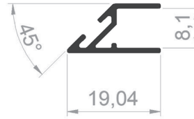
PROFILE CODE: 75420-00 WEIGHT: 0,130 Kg/m
