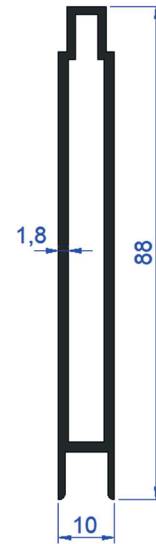
PROFILE CODE: 80001-18 WEIGHT: 0,874 Kg/m
