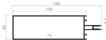
PROFILE CODE: 83060-00 WEIGHT: 2,605 Kg/m
