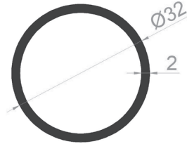
PROFILE CODE: 35078-00 WEIGHT: 0,511 Kg/m
