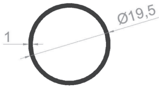
PROFILE CODE: 35019-00 WEIGHT: 0,156 Kg/m
