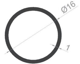
PROFILE CODE: 35074-00 WEIGHT: 0,128 Kg/m
