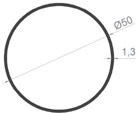
PROFILE CODE: 50379-00 WEIGHT: 0,539 kg/m
