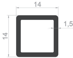
PROFILE CODE: 50135-00 WEIGHT: 0,201 Kg/m
