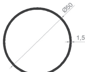
PROFILE CODE: 50295-00 WEIGHT: 0,619 kg/m
