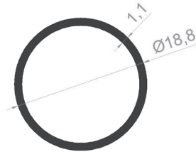
PROFILE CODE: 35003-00 WEIGHT: 0,166 Kg/m
